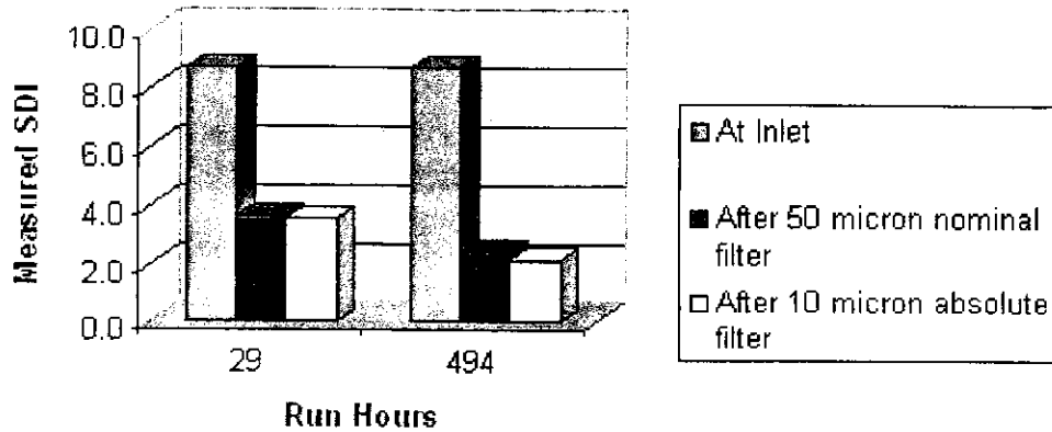
Fig. 7 Measured SDI vs Run Hours for the Two Filters in Series Process (4/27/05 - 5/18/05)
