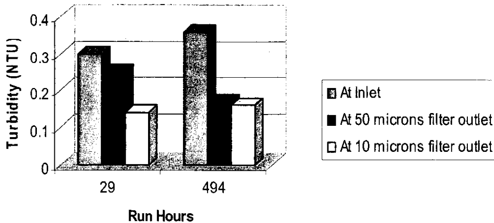
Fig. 7A Measured Seawater Turbidity vs Run Hours
