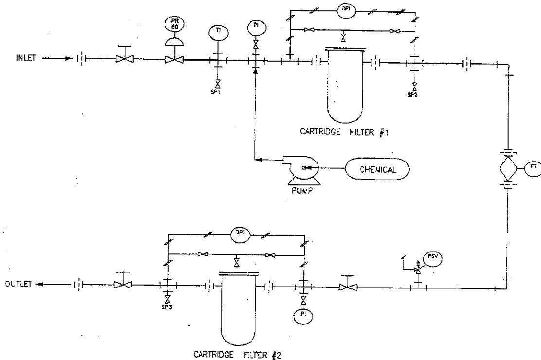
Fig. 1 Pilot Skid Layout
