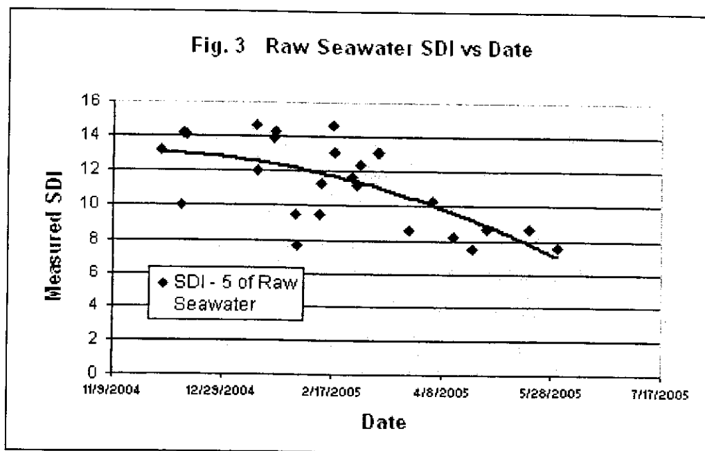
Fig. 3 Measured Feed Seawater SDI vs. Run Date
